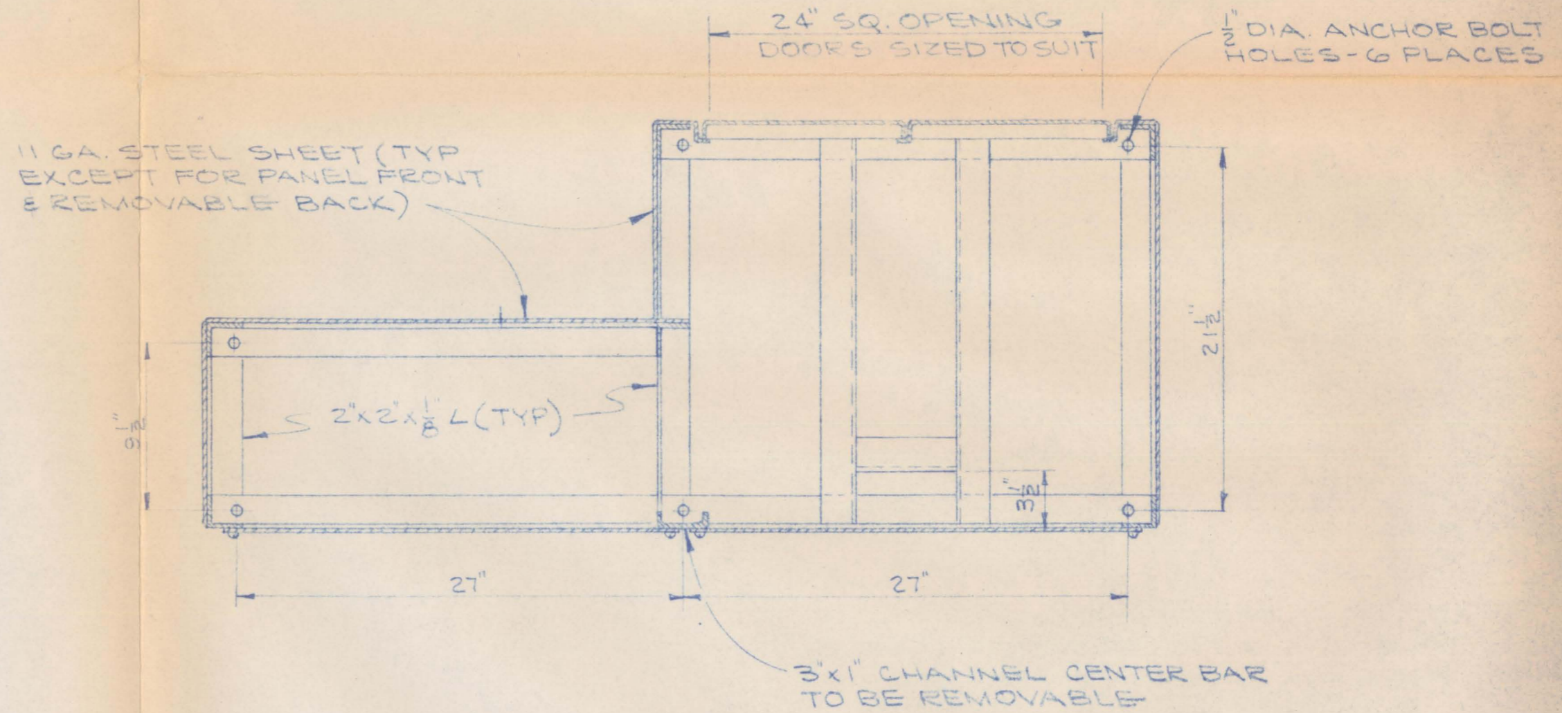
SECTION B-B
